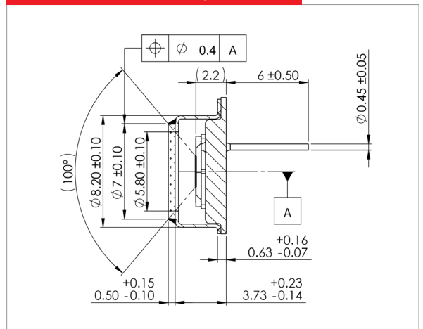
Sectional – JSIR 350-4 cap with filter
